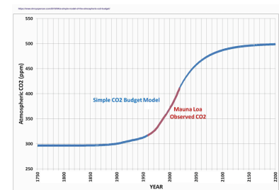
Roy Spencer Atmospheric CO2 budget
